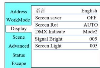
Figure 6-3 Display Settings
